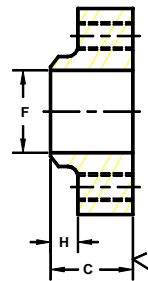
FLAT-FACED 1122 1124
