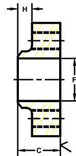
FLAT-FACED 1400 1402
